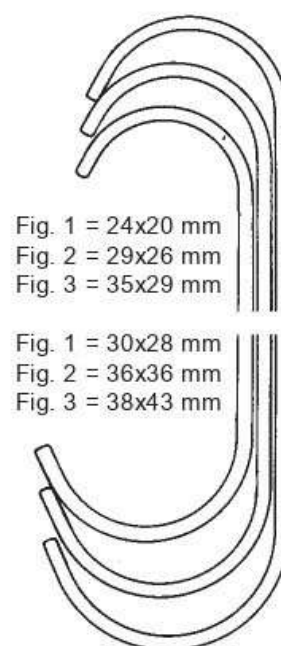
19120-14 Fig. 1 14 cm, 5 1/2" 19120-15 Fig. 2 15 cm, 6" 19120-17 Fig. 3 17 cm, 6 3/4"
